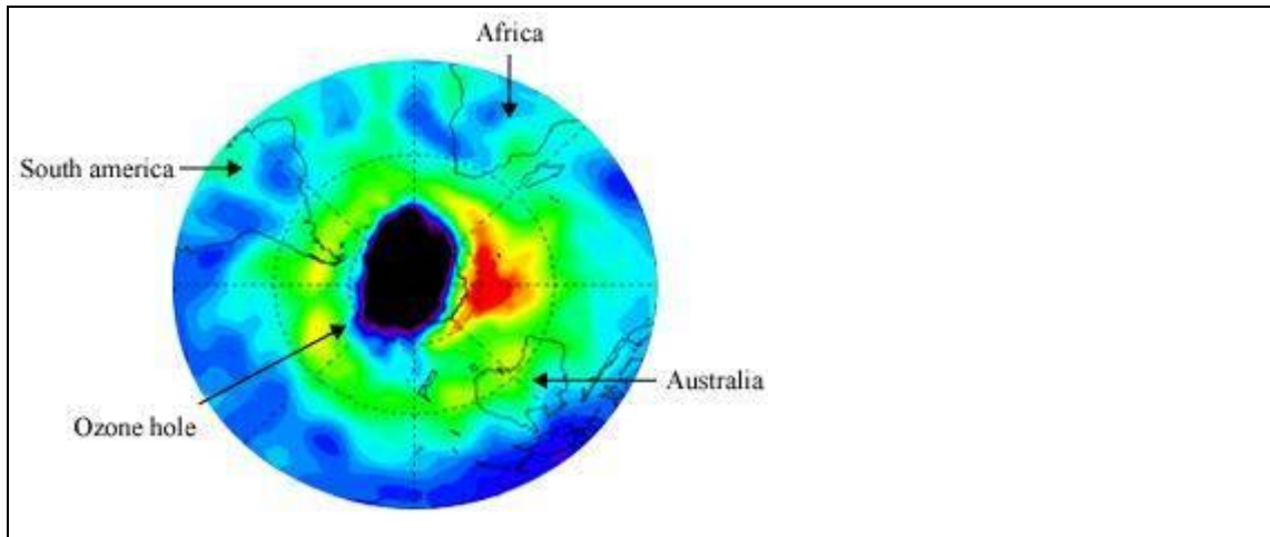
Diagram representing ozone hole
